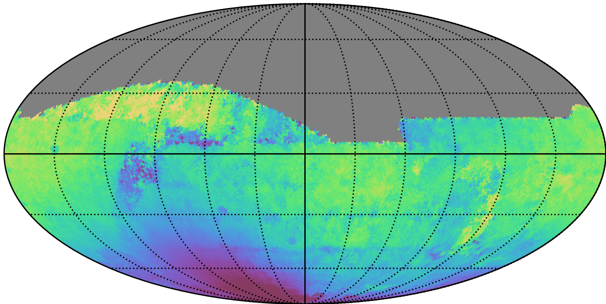
too_ignore_10_4v3.4_10yrs All sky z band: Median solarElong
