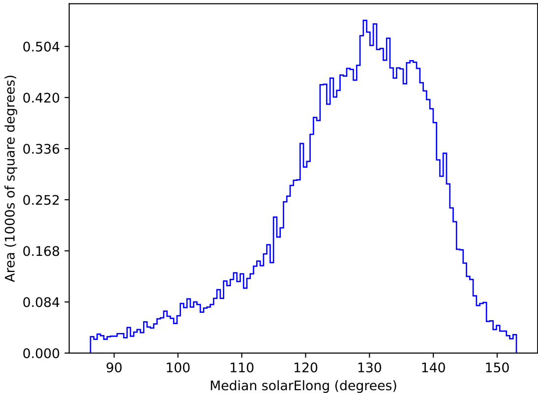
too_ignore_10_4v3.4_10yrs All sky z band: Median solarElong
