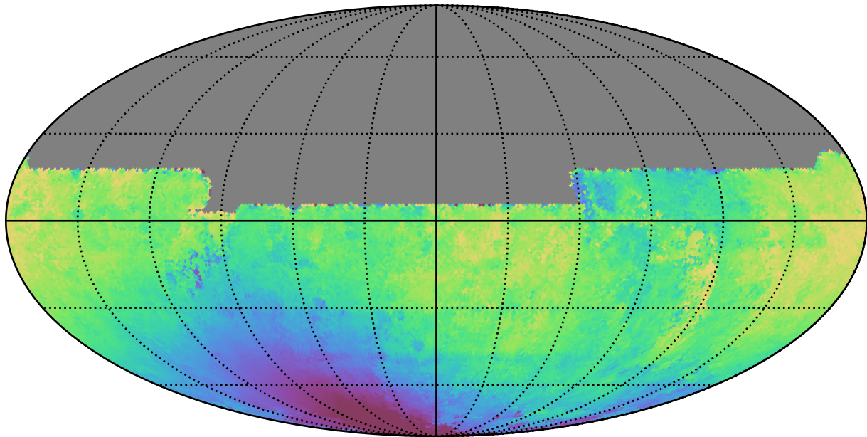
too_ignore_10_4v3.4_10yrs All sky y band: Median solarElong
