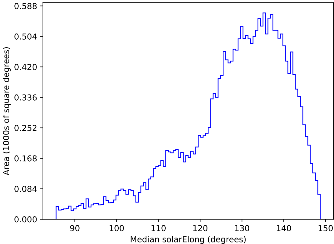
too_ignore_10_4v3.4_10yrs All sky y band: Median solarElong
