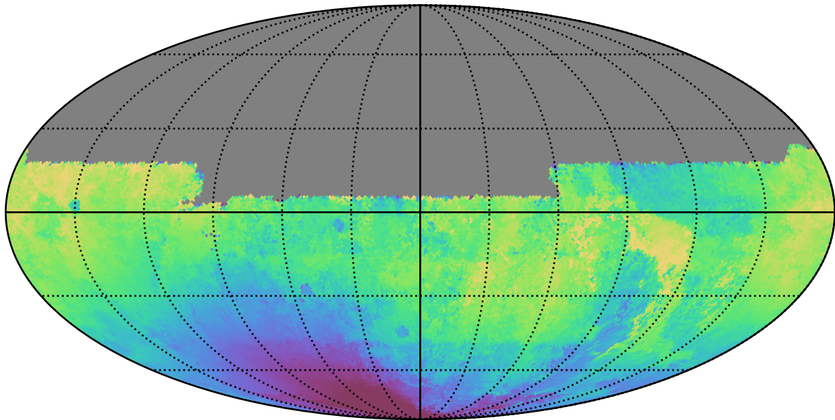
too_ignore_10_4v3.4_10yrs All sky u band: Median solarElong
