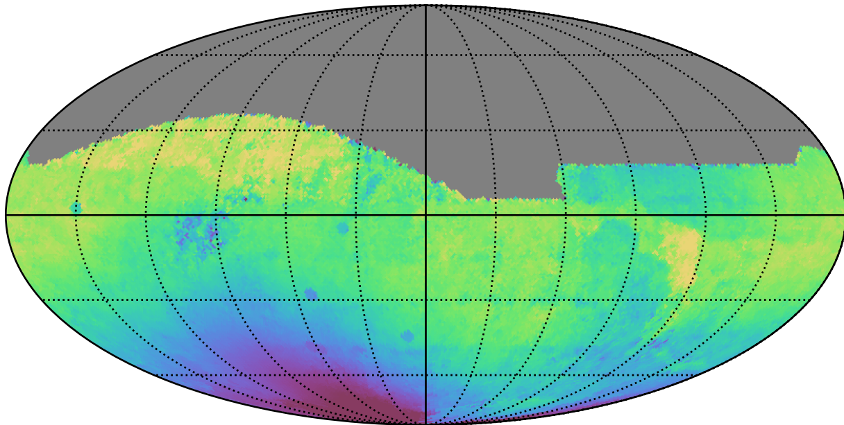
too_ignore_10_4v3.4_10yrs All sky r band: Median solarElong
