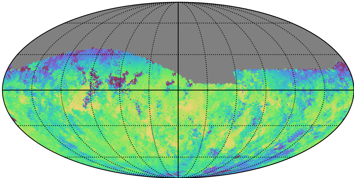
too_ignore_10_4v3.4_10yrs Yr 1 z band: Median skyBrightness
