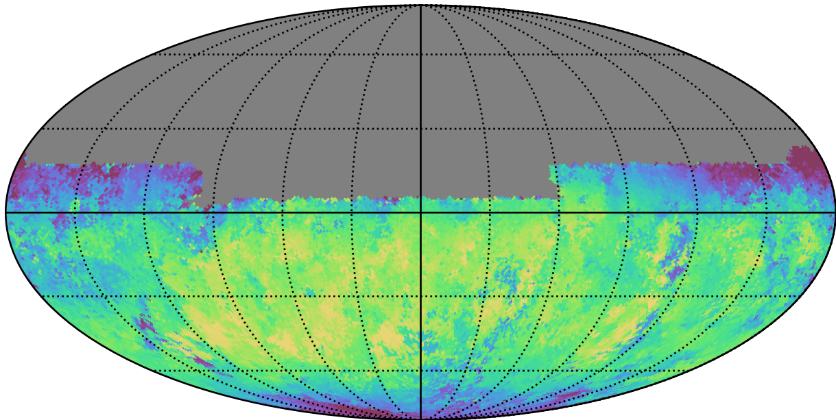
too_ignore_10_4v3.4_10yrs Yr 1 y band: Median skyBrightness
