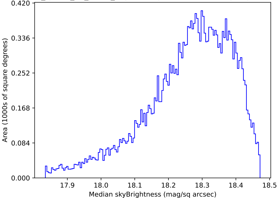
too_ignore_10_4v3.4_10yrs Yr 1 y band: Median skyBrightness
