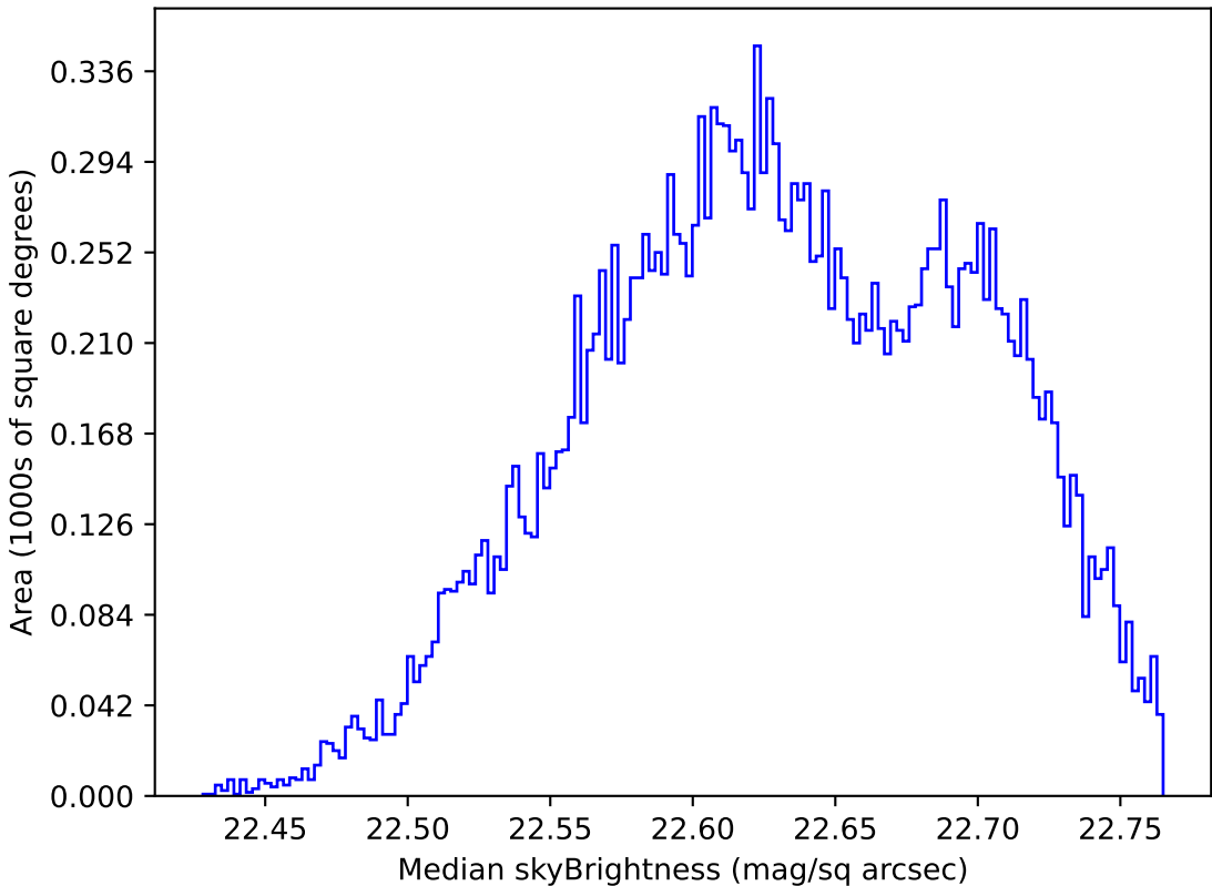
too_ignore_10_4v3.4_10yrs Yr 1 u band: Median skyBrightness
