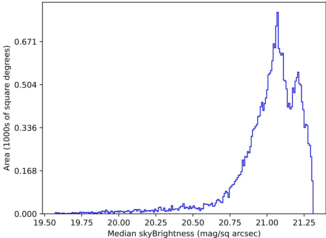
too_ignore_10_4v3.4_10yrs Yr 1 r band: Median skyBrightness
