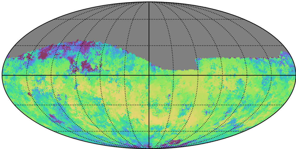
too_ignore_10_4v3.4_10yrs Yr 1 i band: Median skyBrightness
