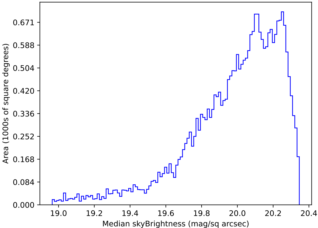
too_ignore_10_4v3.4_10yrs Yr 1 i band: Median skyBrightness
