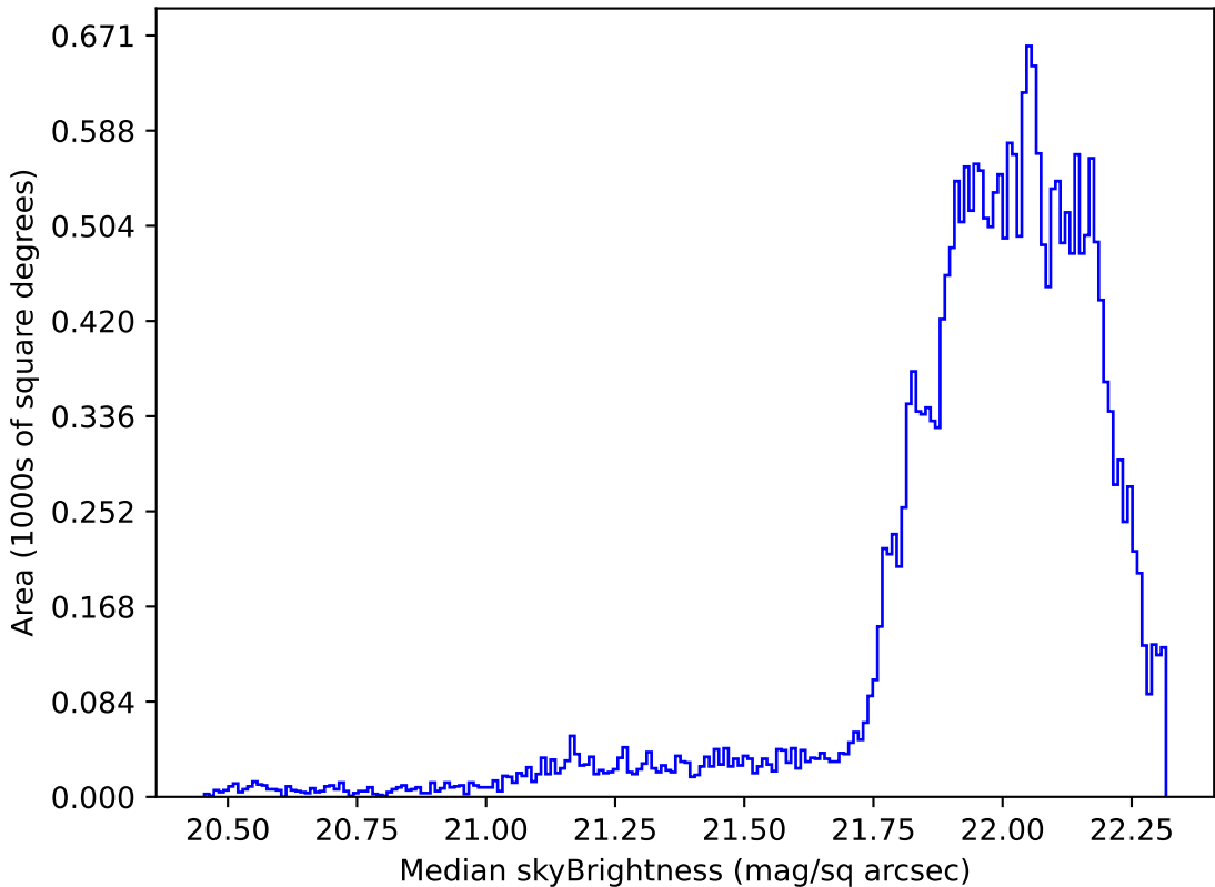
too_ignore_10_4v3.4_10yrs Yr 1 g band: Median skyBrightness
