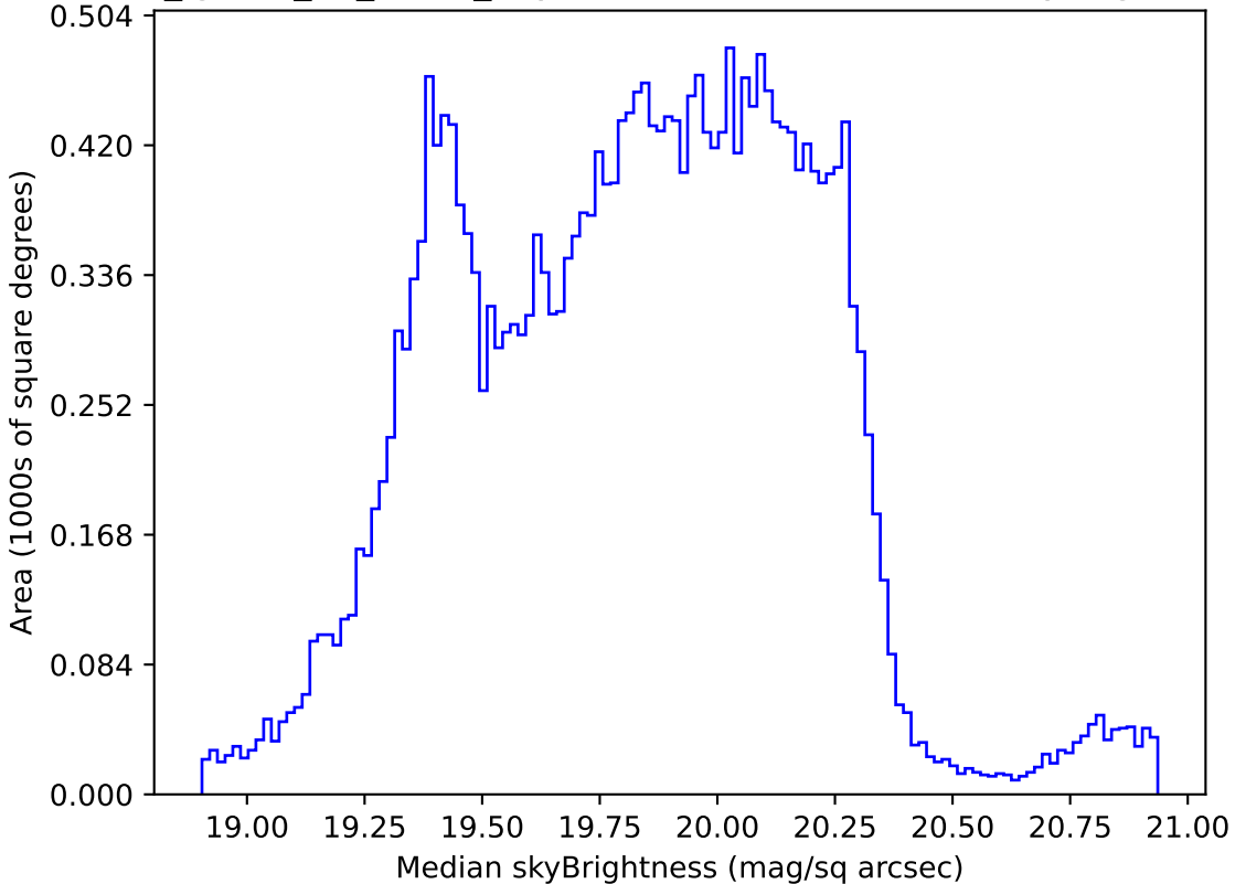
too_ignore_10_4v3.4_10yrs Yr 1 all bands: Median skyBrightness
