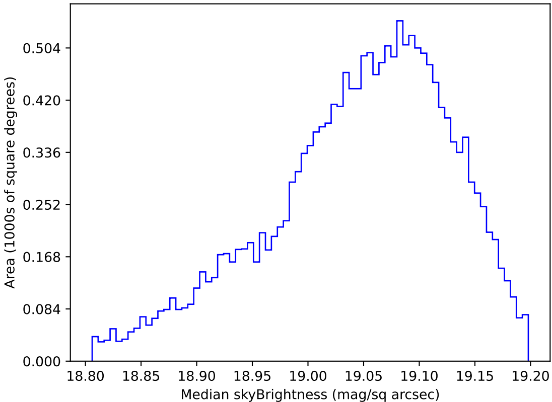
too_ignore_10_4v3.4_10yrs WFD z band: Median skyBrightness
