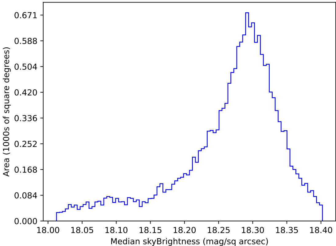
too_ignore_10_4v3.4_10yrs WFD y band: Median skyBrightness
