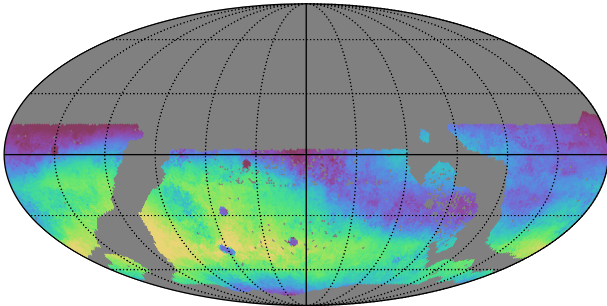
too_ignore_10_4v3.4_10yrs WFD r band: Median skyBrightness
