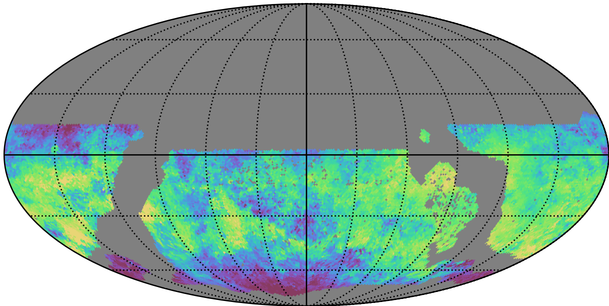
too_ignore_10_4v3.4_10yrs WFD i band: Median skyBrightness
