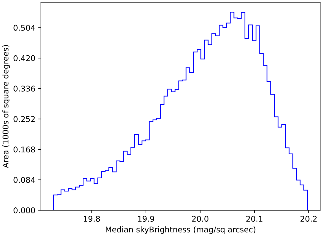
too_ignore_10_4v3.4_10yrs WFD i band: Median skyBrightness
