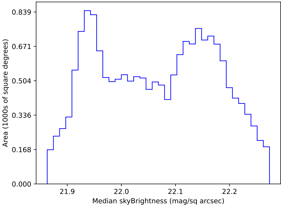
too_ignore_10_4v3.4_10yrs WFD g band: Median skyBrightness
