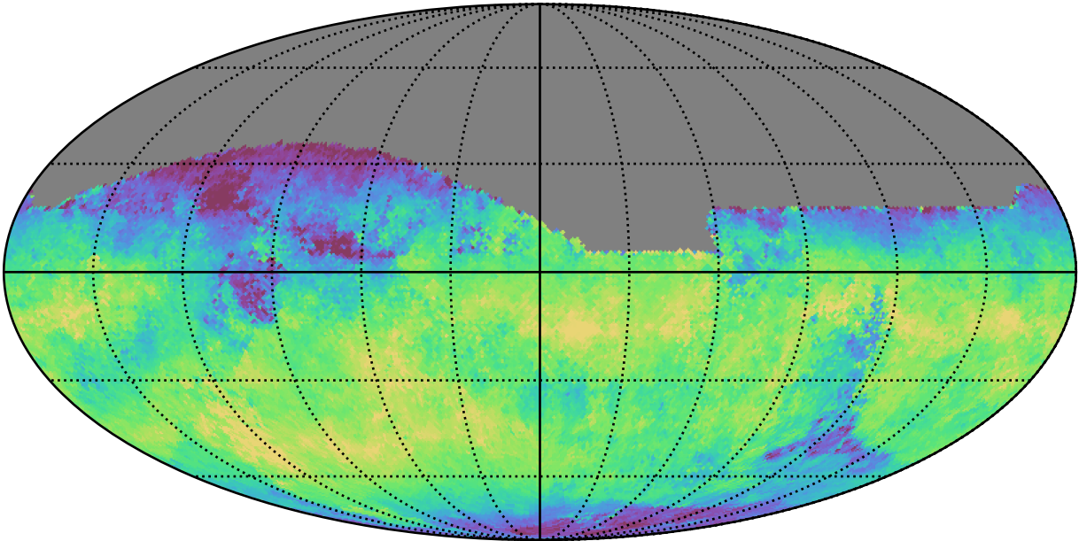
too_ignore_10_4v3.4_10yrs All sky z band: Median skyBrightness
