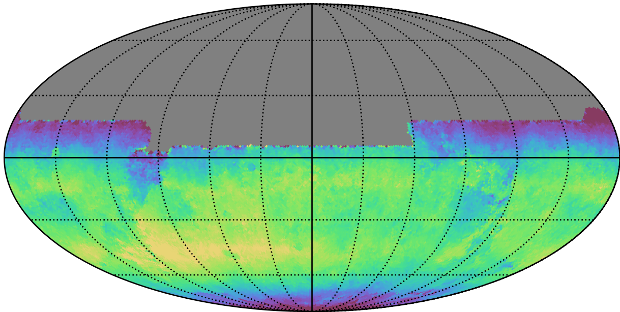
too_ignore_10_4v3.4_10yrs All sky y band: Median skyBrightness
