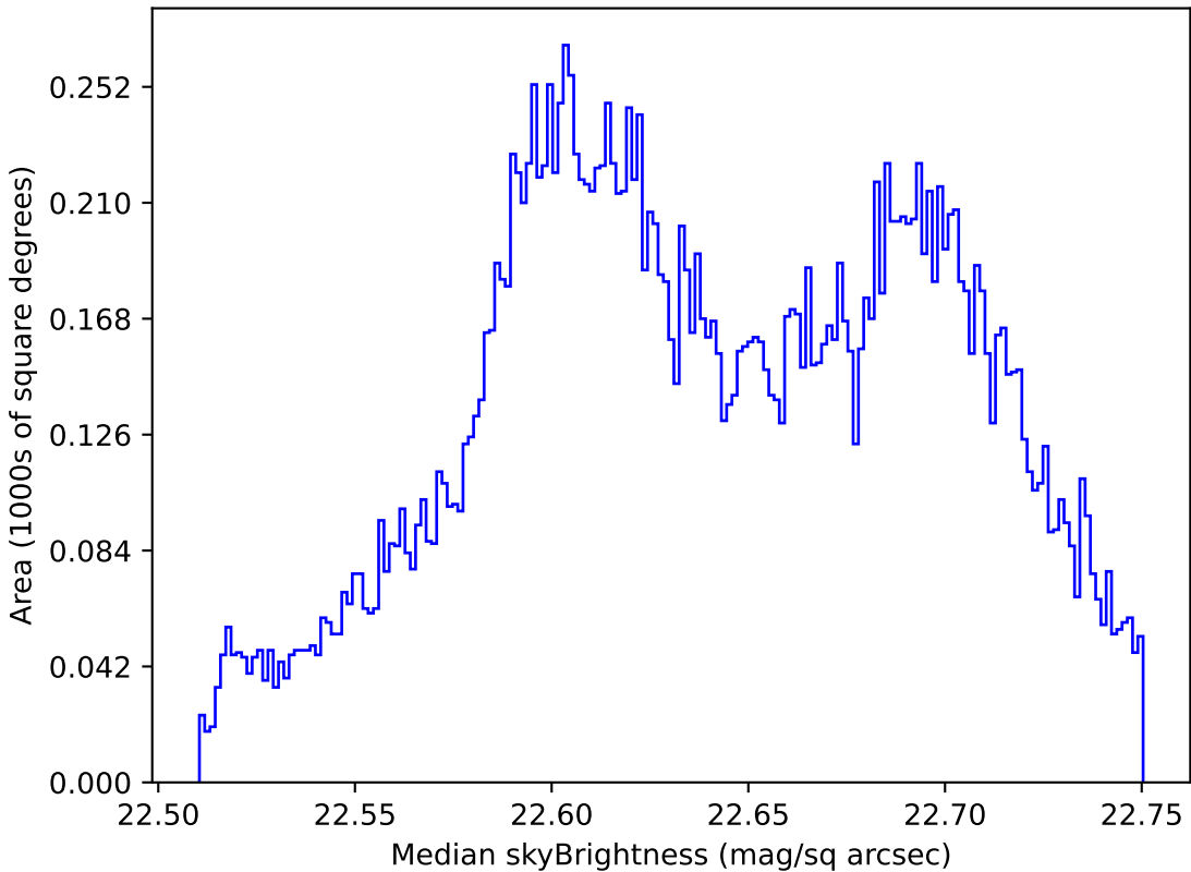
too_ignore_10_4v3.4_10yrs All sky u band: Median skyBrightness
