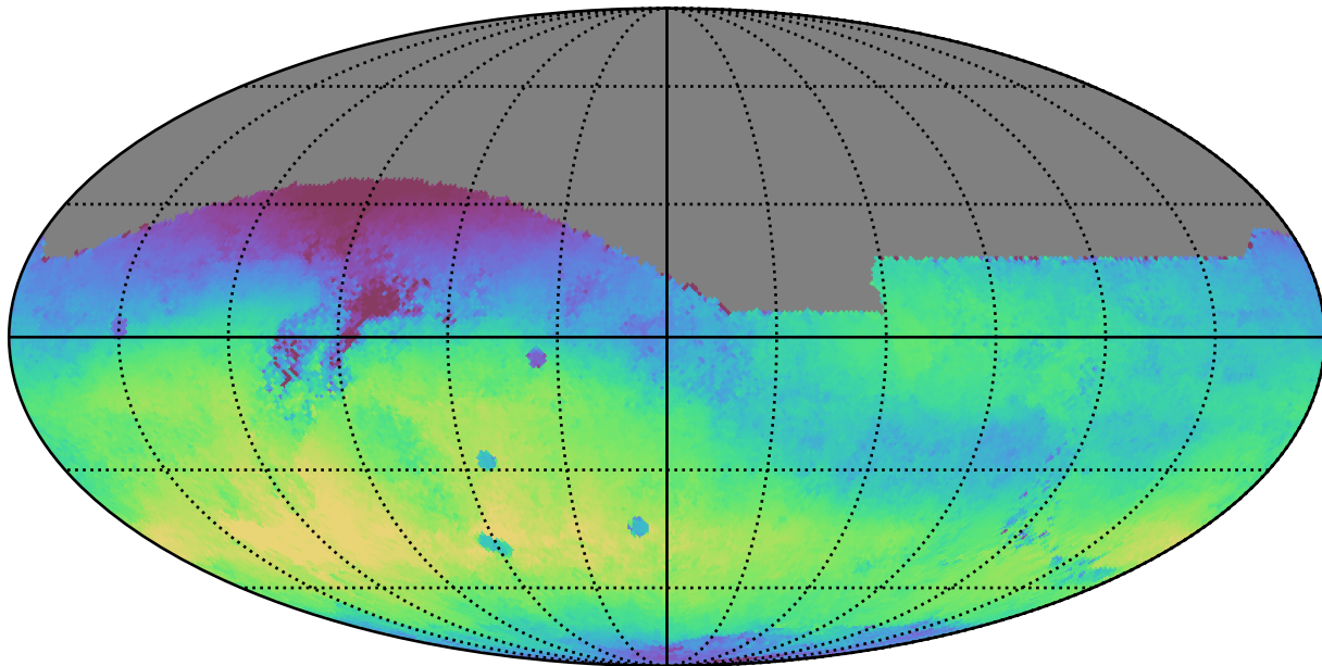
too_ignore_10_4v3.4_10yrs All sky r band: Median skyBrightness
