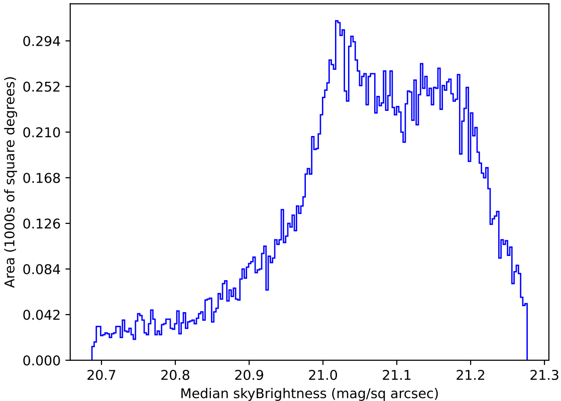
too_ignore_10_4v3.4_10yrs All sky r band: Median skyBrightness
