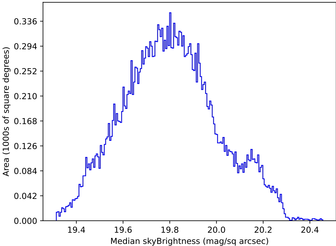
too_ignore_10_4v3.4_10yrs All sky all bands: Median skyBrightness
