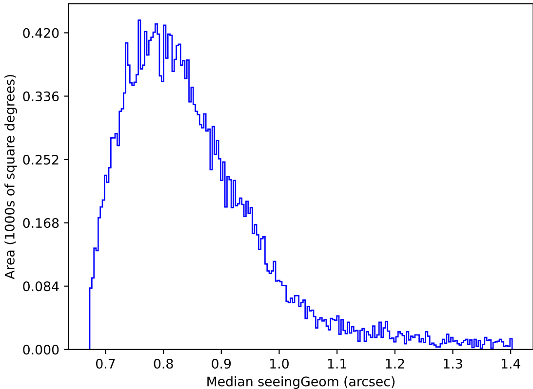
too_ignore_10_4v3.4_10yrs Yr 1 z band: Median seeingGeom
