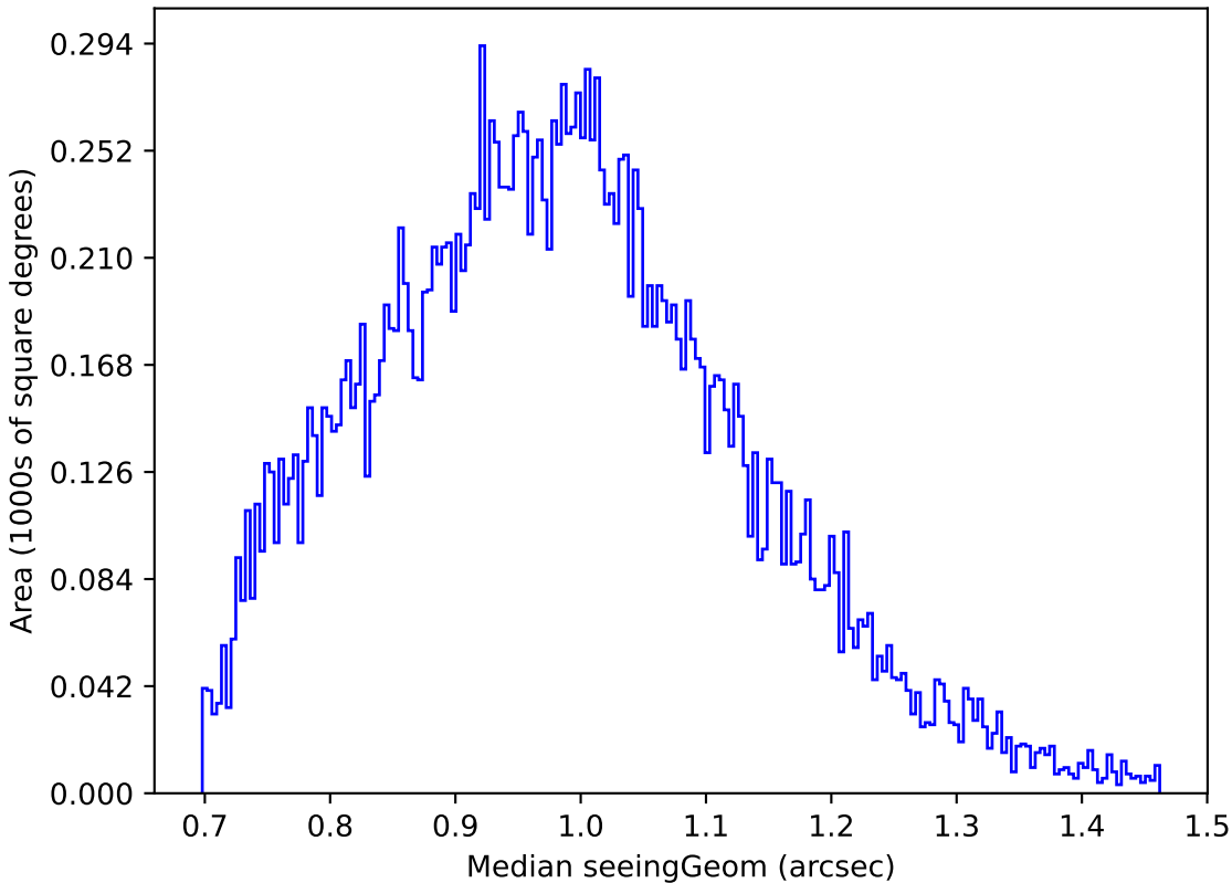
too_ignore_10_4v3.4_10yrs Yr 1 u band: Median seeingGeom
