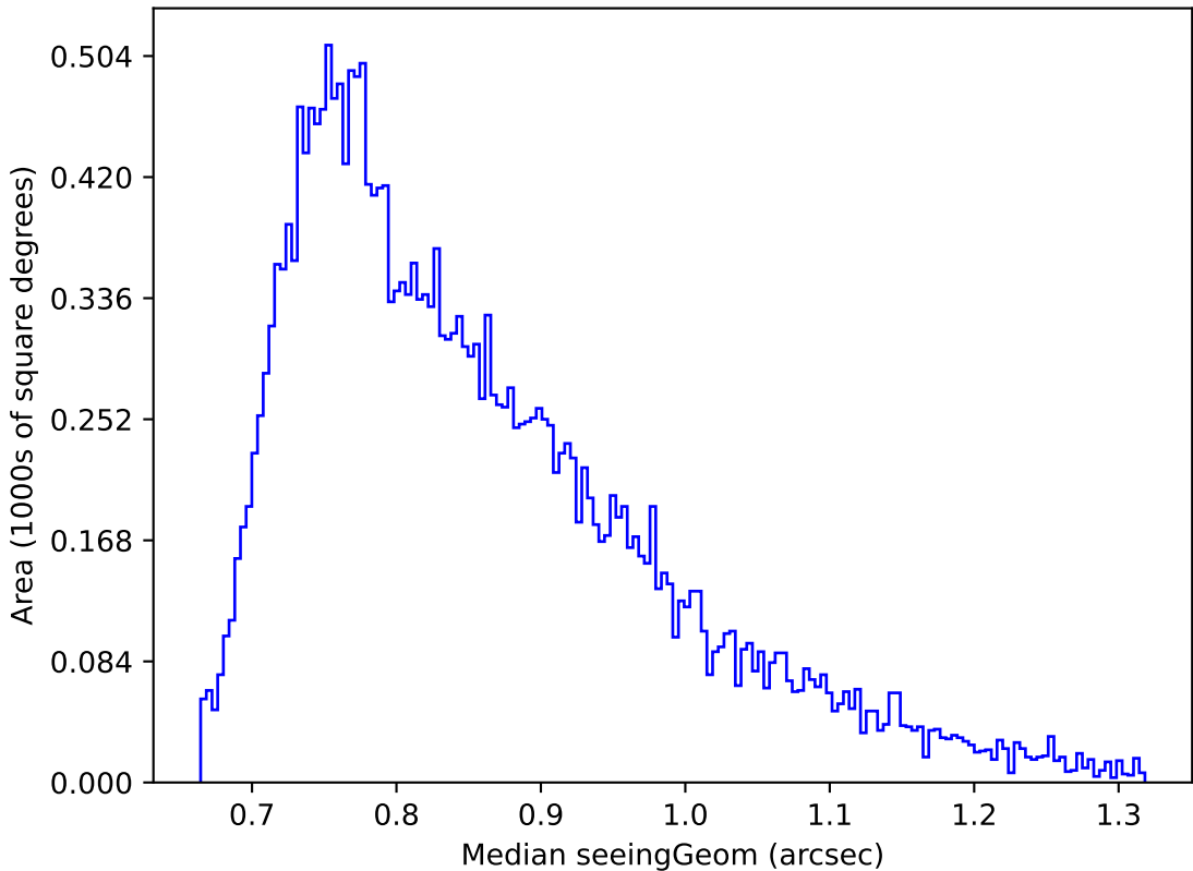
too_ignore_10_4v3.4_10yrs Yr 1 r band: Median seeingGeom
