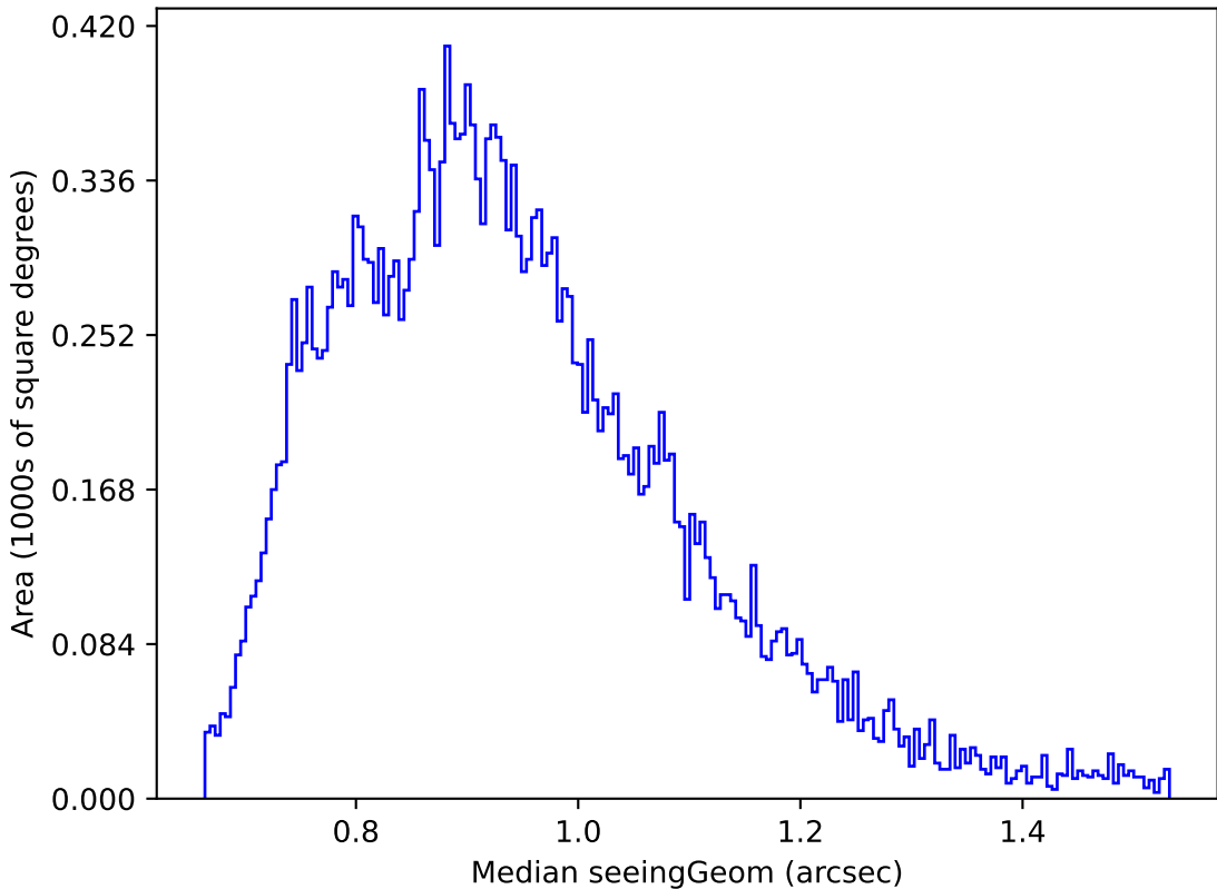
too_ignore_10_4v3.4_10yrs Yr 1 g band: Median seeingGeom
