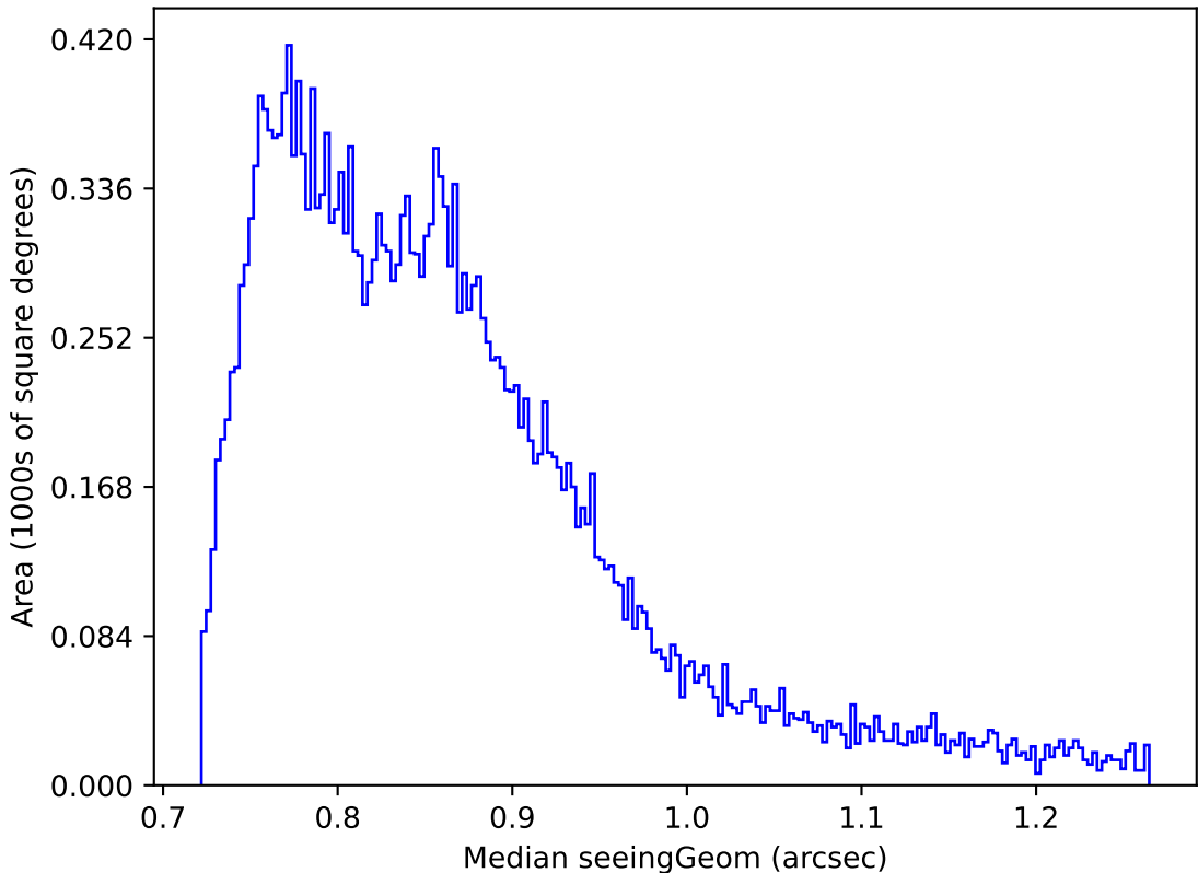
too_ignore_10_4v3.4_10yrs Yr 1 all bands: Median seeingGeom
