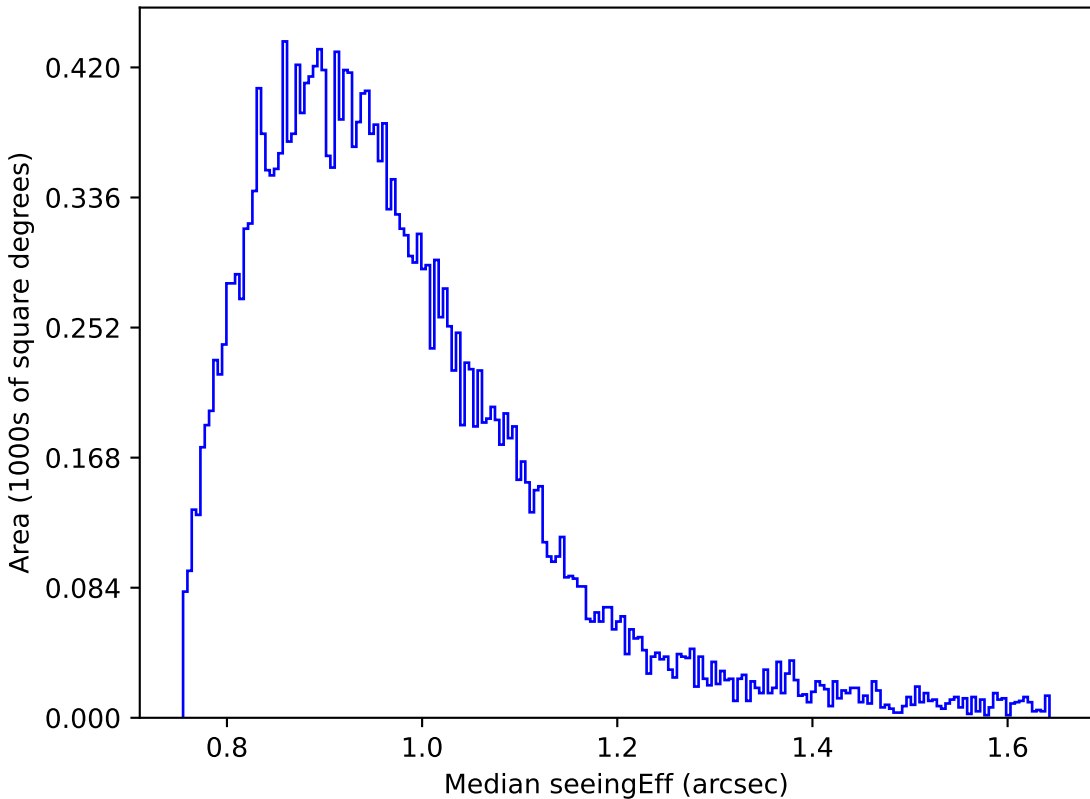
too_ignore_10_4v3.4_10yrs Yr 1 z band: Median seeingEff
