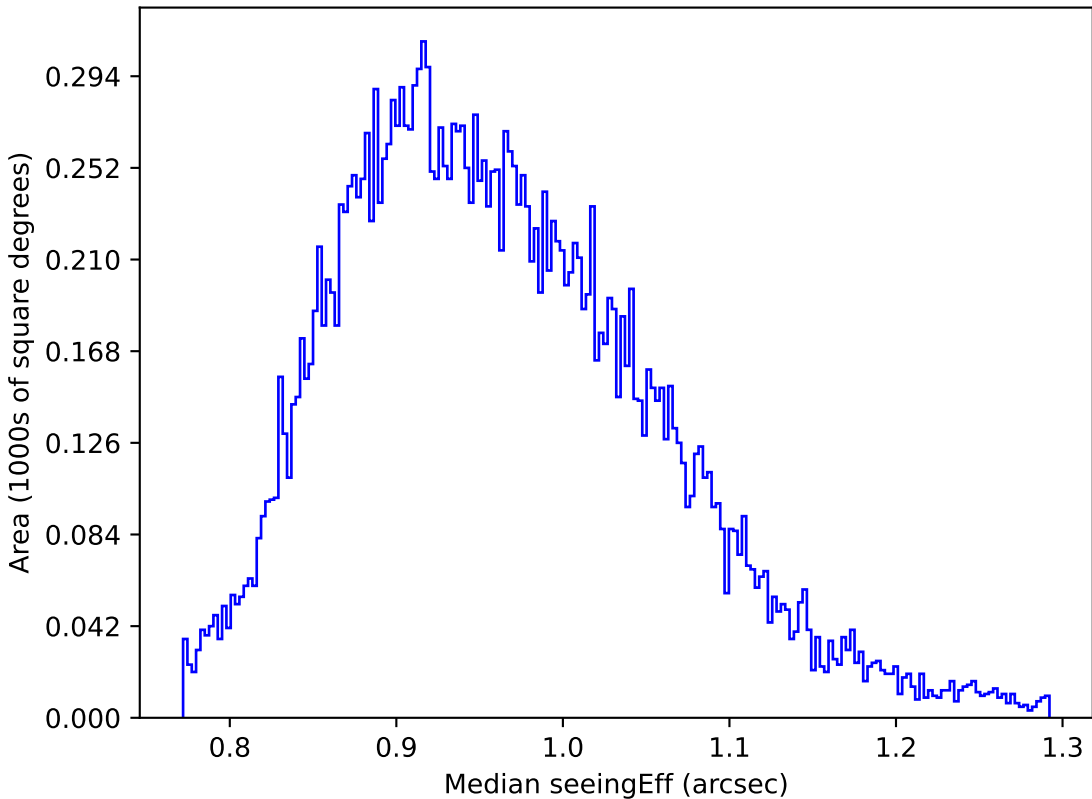
too_ignore_10_4v3.4_10yrs Yr 1 y band: Median seeingEff
