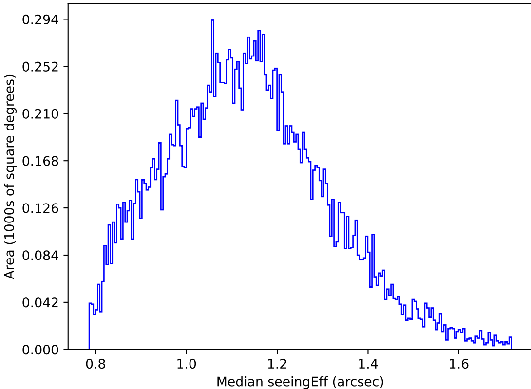
too_ignore_10_4v3.4_10yrs Yr 1 u band: Median seeingEff
