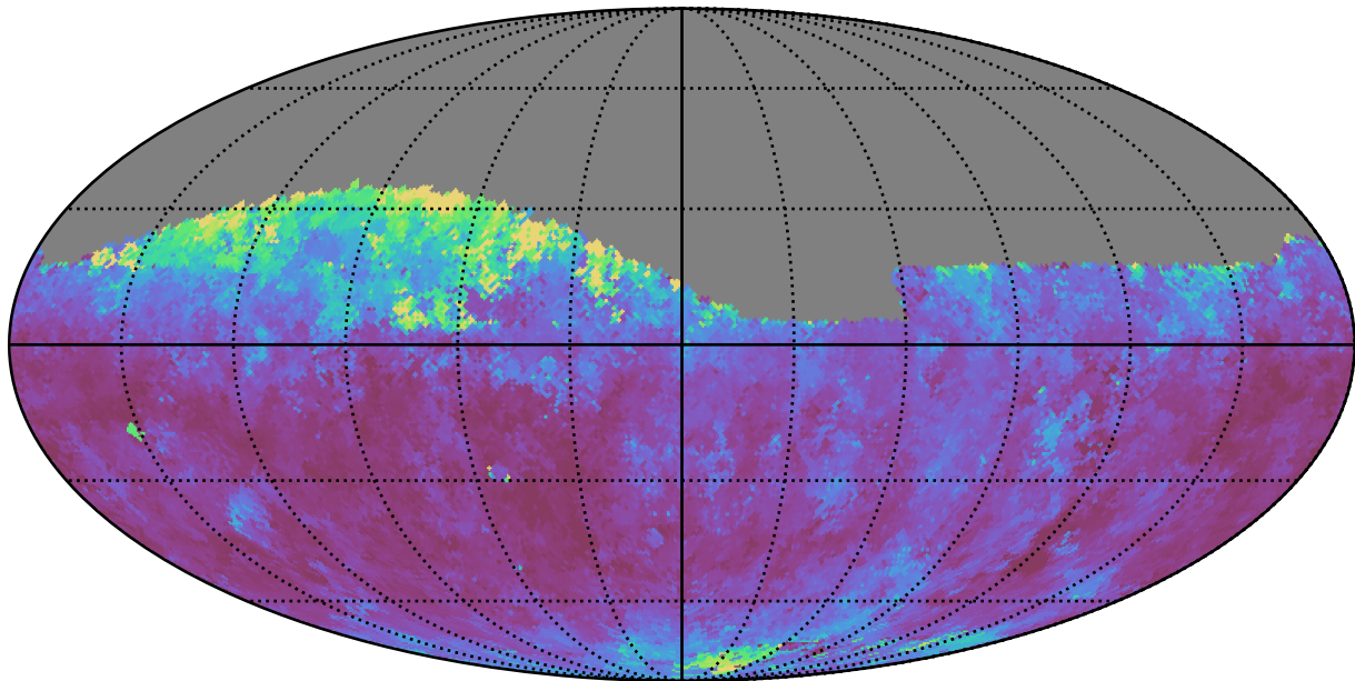
too_ignore_10_4v3.4_10yrs Yr 1 i band: Median seeingEff
