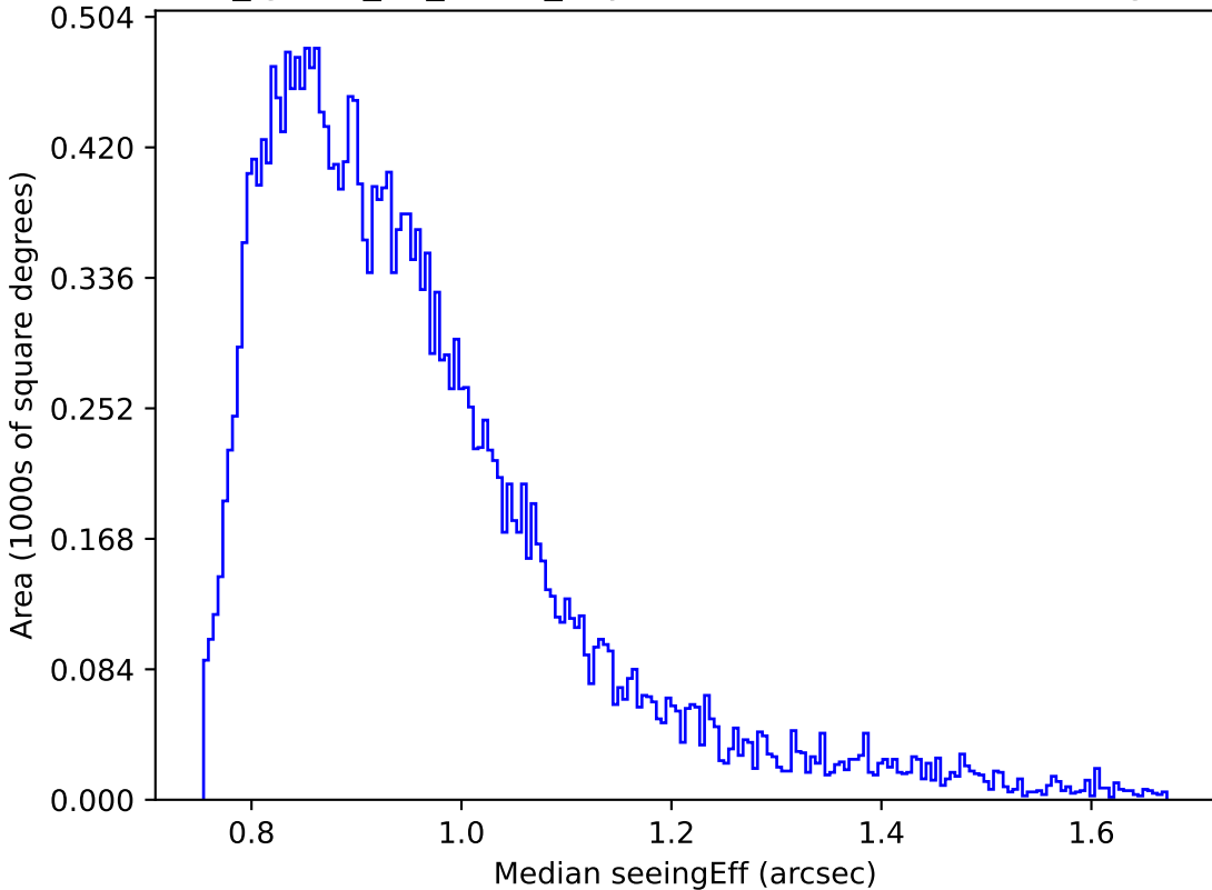
too_ignore_10_4v3.4_10yrs Yr 1 i band: Median seeingEff
