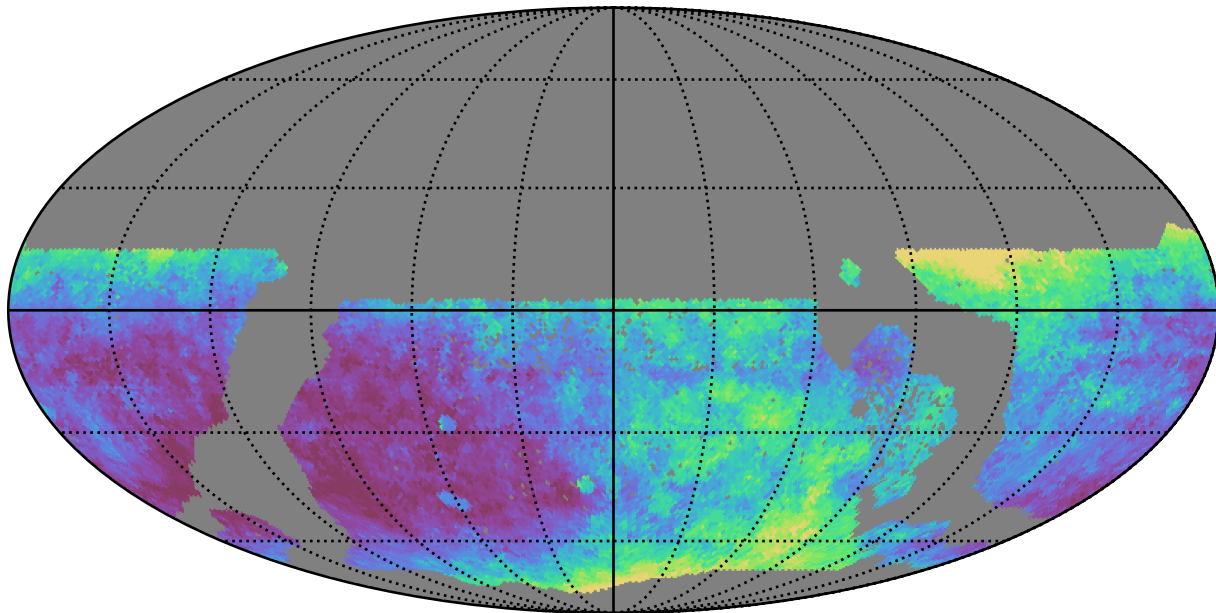
too_ignore_10_4v3.4_10yrs WFD z band: Median seeingEff
