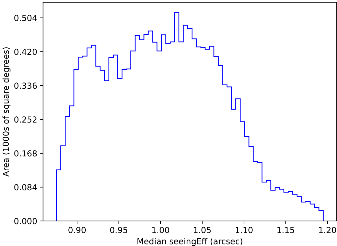
too_ignore_10_4v3.4_10yrs WFD z band: Median seeingEff
