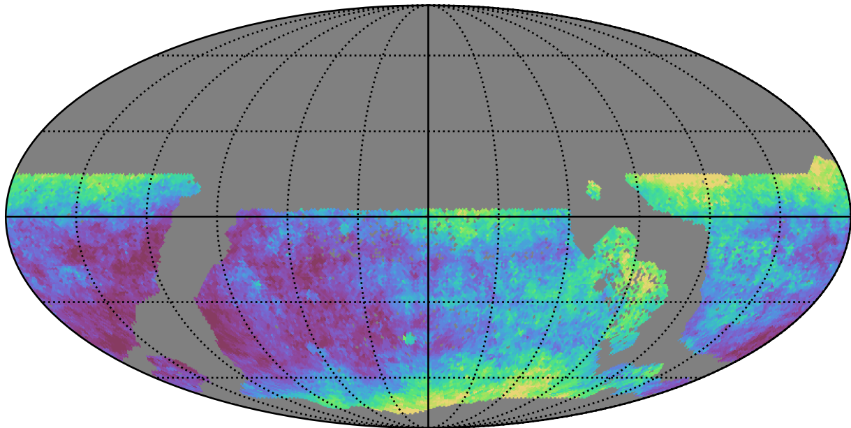
too_ignore_10_4v3.4_10yrs WFD y band: Median seeingEff
