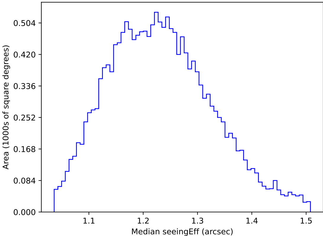
too_ignore_10_4v3.4_10yrs WFD u band: Median seeingEff
