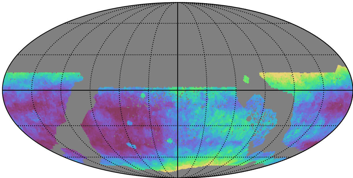
too_ignore_10_4v3.4_10yrs WFD r band: Median seeingEff
