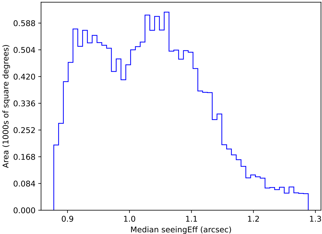
too_ignore_10_4v3.4_10yrs WFD r band: Median seeingEff
