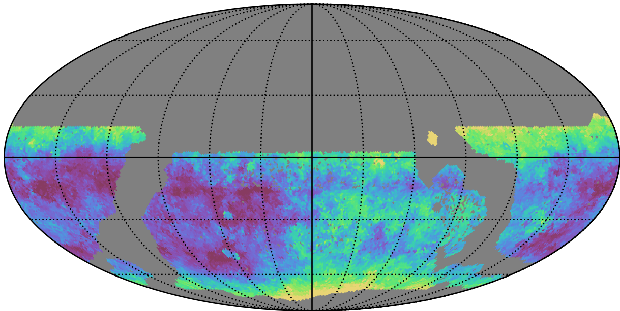
too_ignore_10_4v3.4_10yrs WFD g band: Median seeingEff
