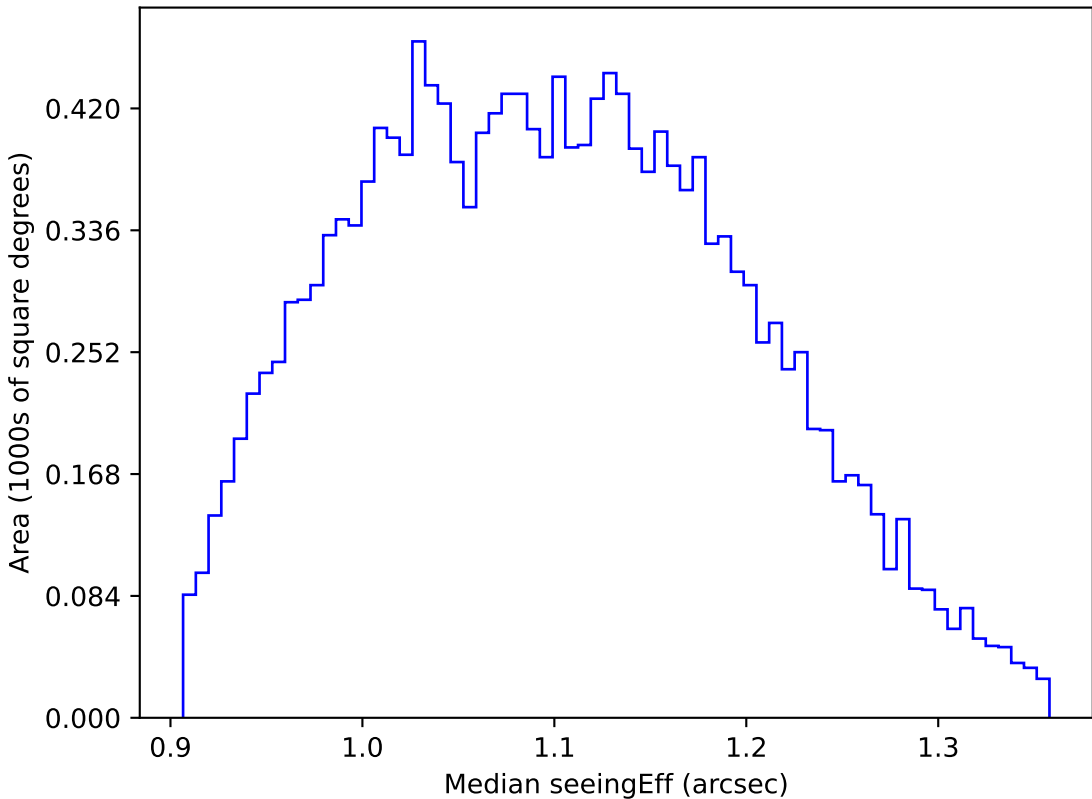
too_ignore_10_4v3.4_10yrs WFD g band: Median seeingEff
