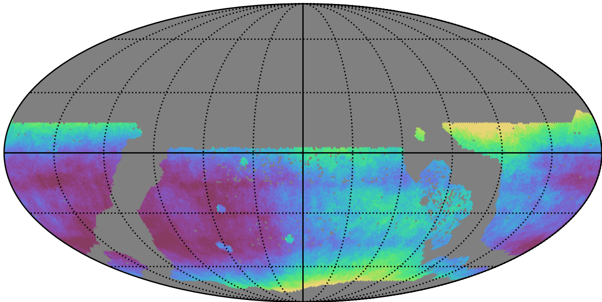
too_ignore_10_4v3.4_10yrs WFD all bands: Median seeingEff
