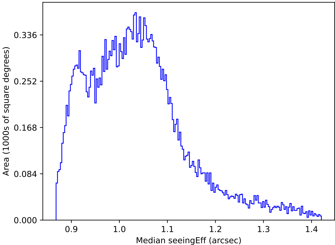
too_ignore_10_4v3.4_10yrs All sky z band: Median seeingEff
