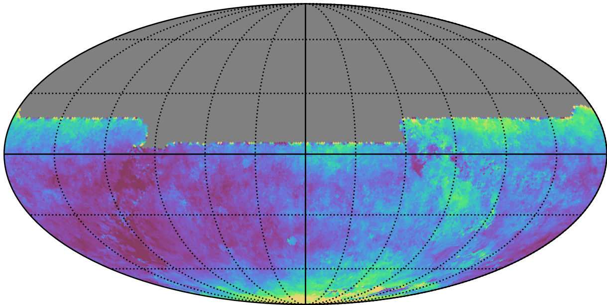
too_ignore_10_4v3.4_10yrs All sky y band: Median seeingEff
