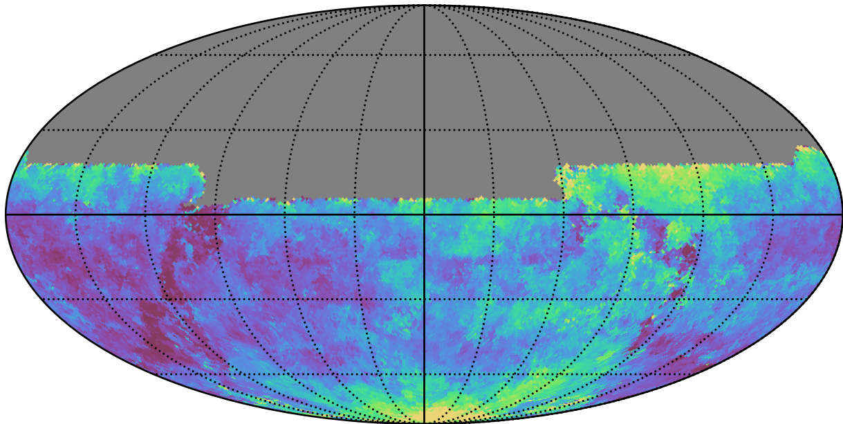
too_ignore_10_4v3.4_10yrs All sky u band: Median seeingEff
