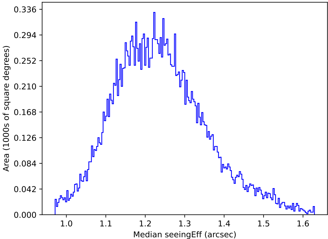
too_ignore_10_4v3.4_10yrs All sky u band: Median seeingEff
